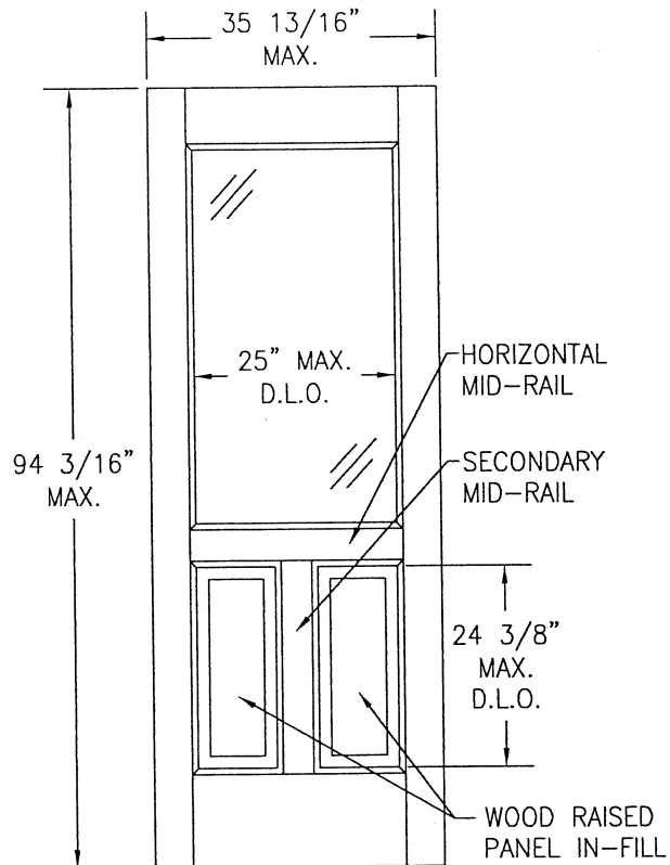
ALTERNATE MID-RAIL & WOOD IN-FILL PANEL CONDITION
