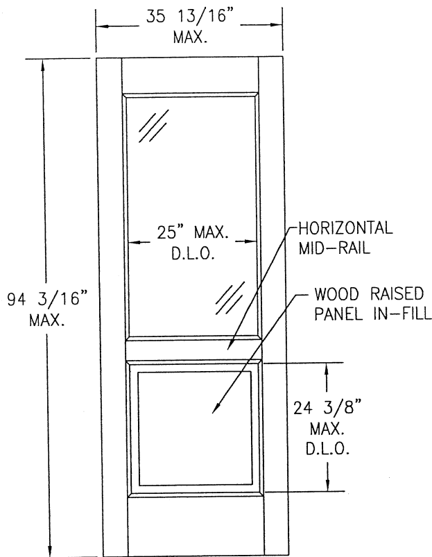
TESTED MID-RAIL & WOOD IN-FILL PANEL CONDITION
